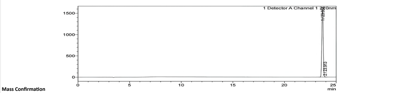
Chromatogram
